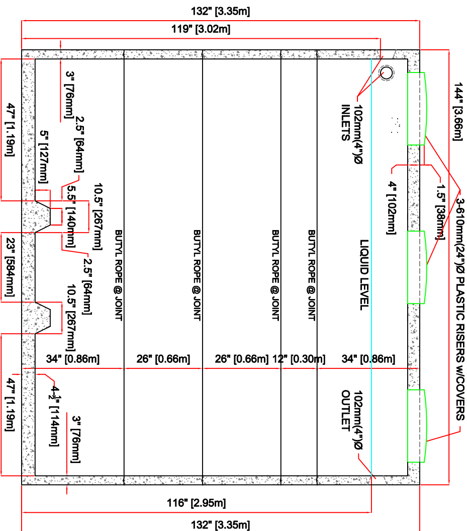
SIDE SECTION
