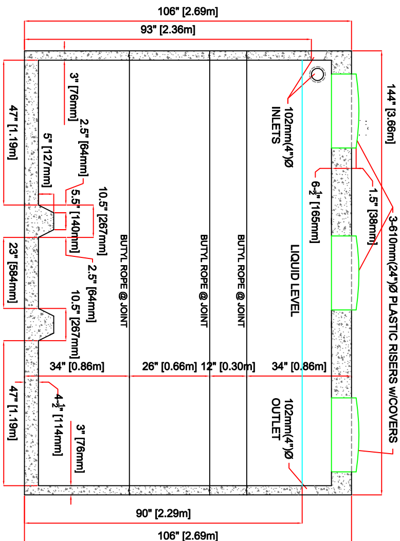
SIDE SECTION
