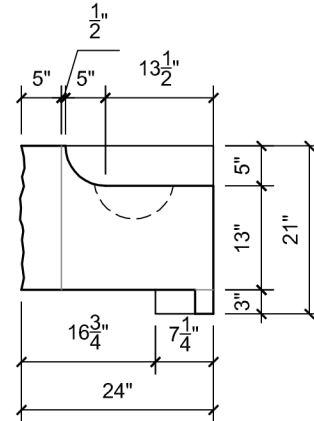
RIGHT END VIEW
